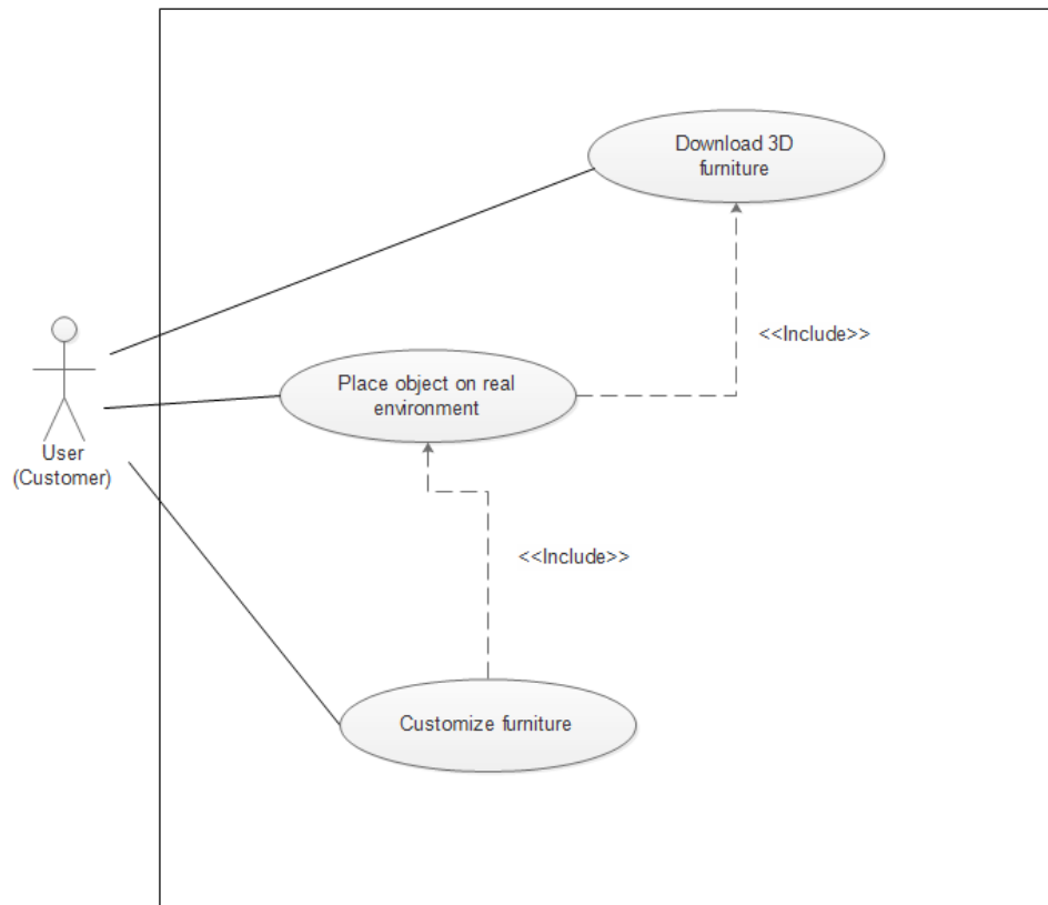
Figure 4.1.1 User-case Diagram
